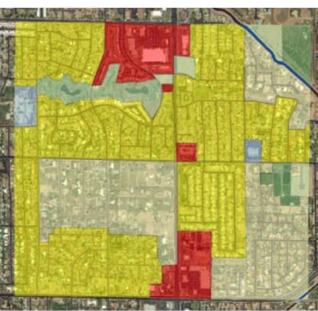
2010 Land Use
