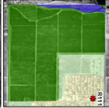
1980 Land Use
