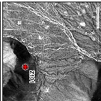
1990 Aerial
