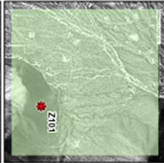
1990 Land Use
