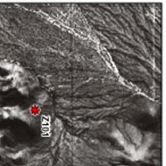
1970 Aerial
