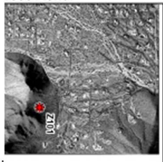
2000 Aerial
