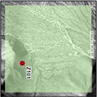
1980 Land Use
