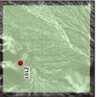
1970 Land Use
