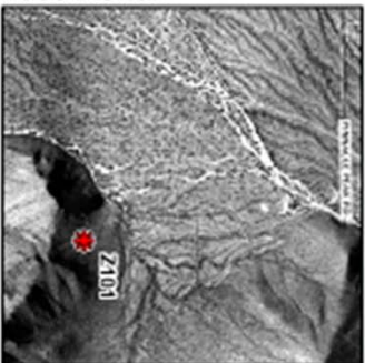
1980 Aerial
