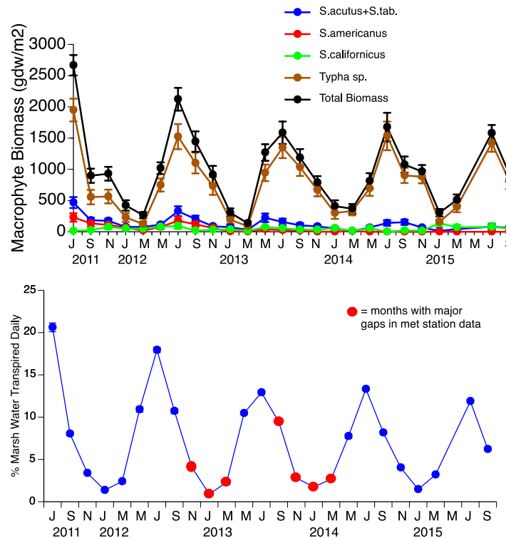
Figure 1.7. Temporal patterns of marsh plant biomass (top) and the fraction of total water overlying the marsh that is lost to plant transpiration daily (bottom), which creates a “biological tide” drawing water and nutrients into the vegetated wetland.
