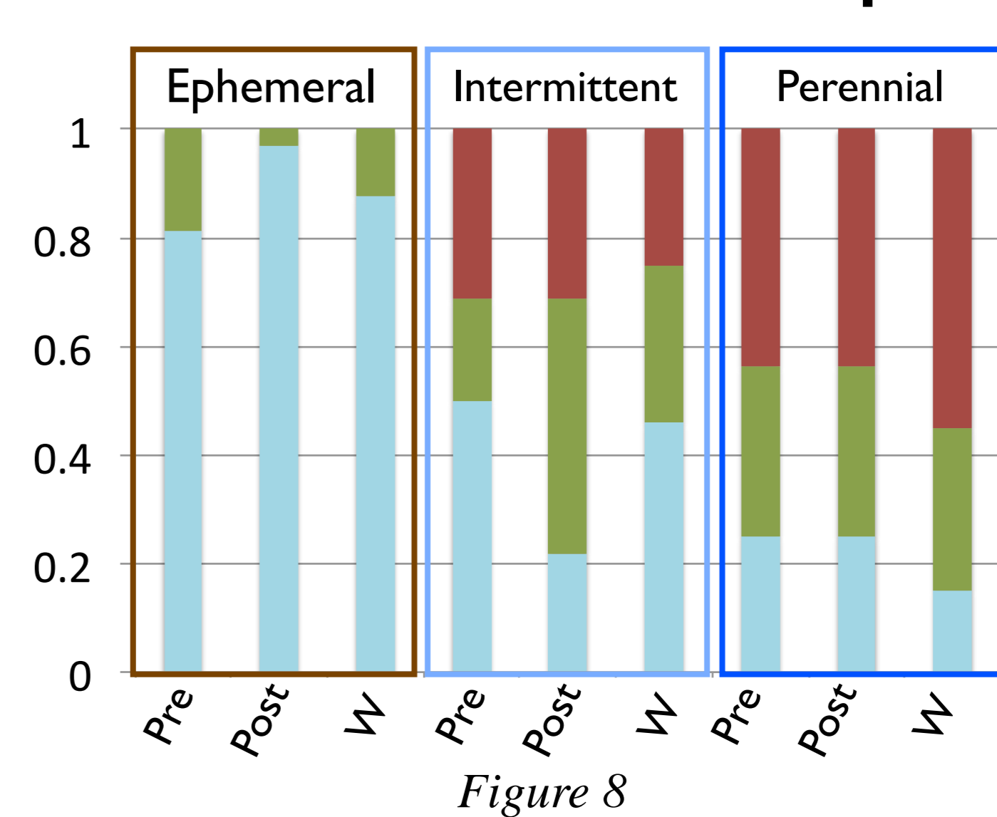
Figure 8 denotes where and when “hotspots” of denitrification potentials occur for all wetlands.
